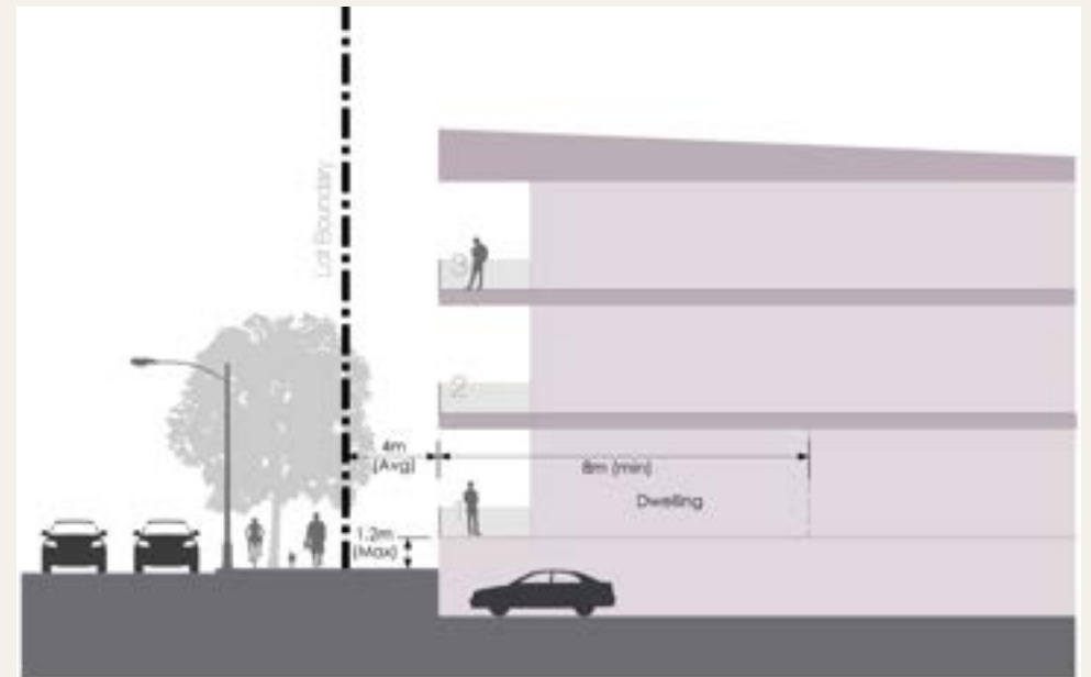
FIGURE 12: RESIDENTIAL 1 R-AC0 BASEMENT PARKING - NIL SETBACKS TO STREET BOUNDARY (APPROPRIATE SCREENING SHALL BE PROVIDED TO CAR PARKS)
