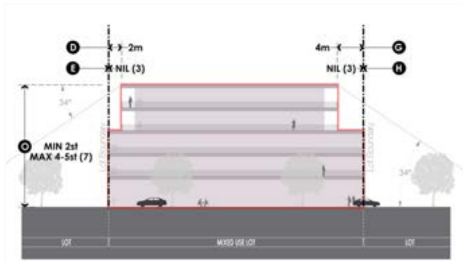
Front View from Scarborough Beach Road - illustrating Building Setbacks and Envelope
