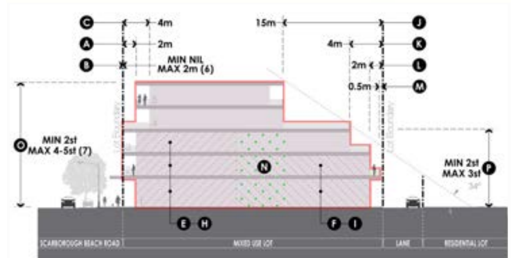
Side View - illustrating Building Setbacks and Envelope
