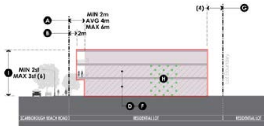
Side View - illustrating Building Setbacks and Envelope
